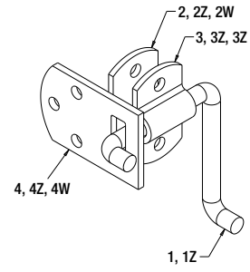
Corner Security Latch
