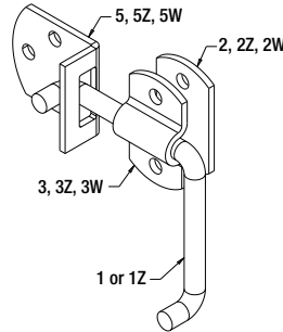
Straight Side Security Latch
