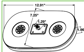
Permanent mounting stud and magnetic mounts
