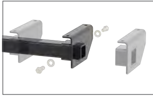
Three-piece, adjustable design fits multiple frame sizes
