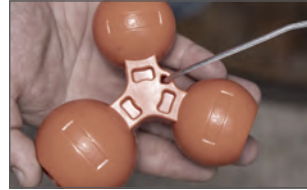
Built-in safety points allow the ball to break off when forcefully tampered with, leaving the ball in the coupler and blocking hookup
